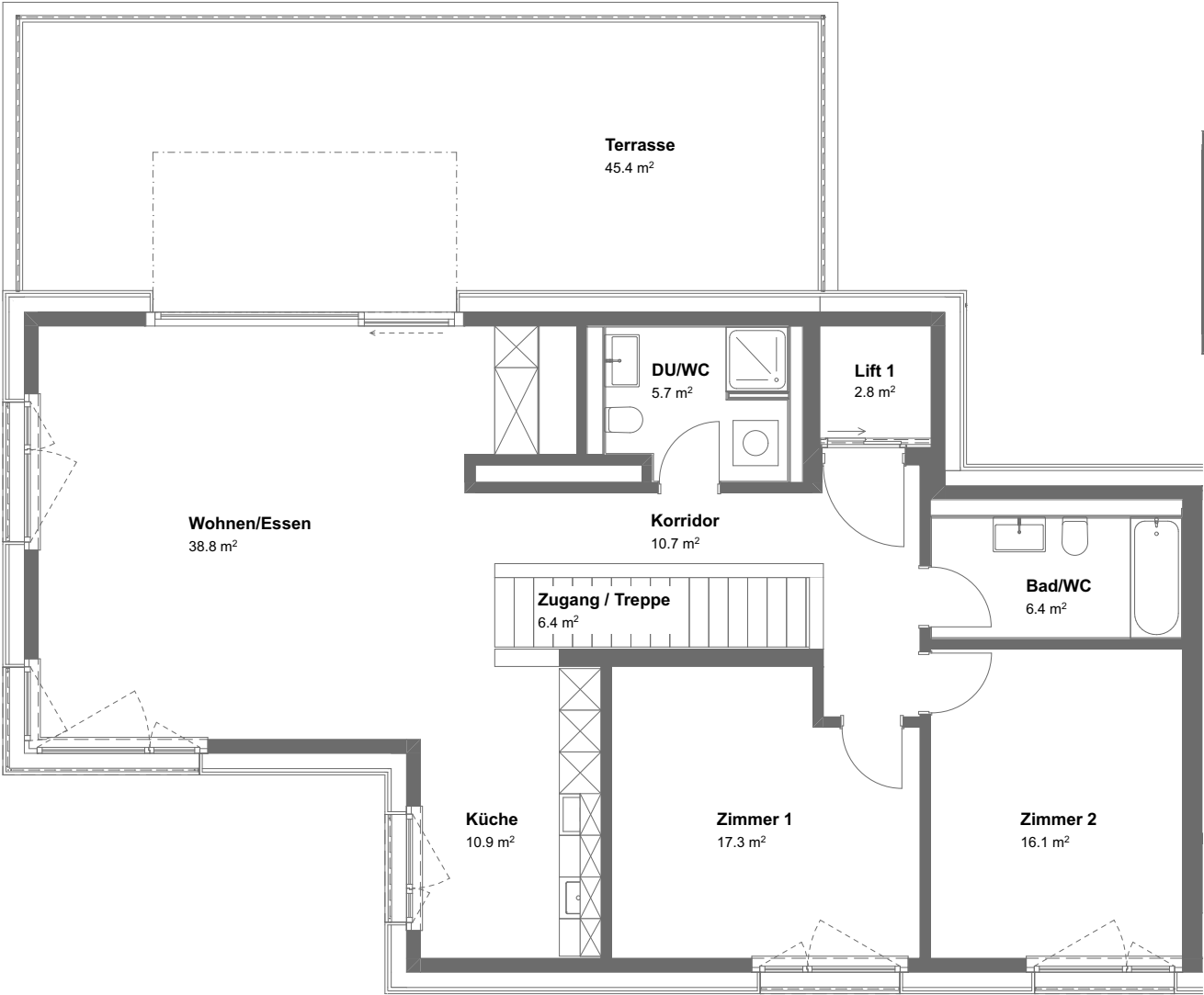
Attikageschoss
